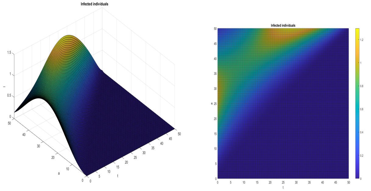
Figure 1. The dynamics of infected population for \alpha = 1 with \mathcal{R}_0 \leq 1 .
