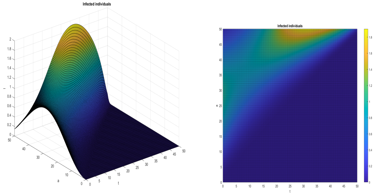
Figure 2. The dynamics of infected population for \alpha = 0.8 with \mathcal{R}_0 \leq 1 .
