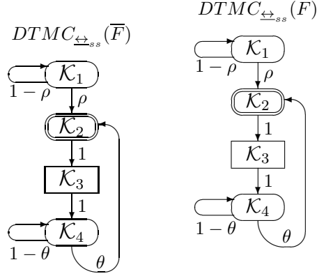
FIG. 8. The quotient DTMC of \bar{F} for F = [(\{a\}, \rho) * ((\{b\}, \mathfrak{d}_k^1); ((\{c\}, \mathfrak{d}_l^0); (\{d\}, \theta)_1)[((\{c\}, \mathfrak{d}_m^0); (\{d\}, \theta)_2))) * \text{Stop}]
