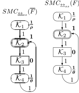
FIG. 6. The quotient underlying SMC of \bar{F} for F = [(\{a\}, \rho) * ((\{b\}, \mathfrak{z}_k^1); (((\{c\}, \mathfrak{z}_l^0); (\{d\}, \theta)_1) \square ((\{c\}, \mathfrak{z}_m^0); (\{d\}, \theta)_2))) * \text{Stop}]
