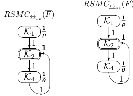
FIG. 10. The reduced quotient SMC of \overline{F} for F = [(\{a\}, \rho) * ((\{b\}, \frac{1}{k}); (((\{c\}, \frac{1}{l}); (\{d\}, \theta)_1) \square ((\{c\}, \frac{1}{m}); (\{d\}, \theta)_2))) * \text{Stop}]
