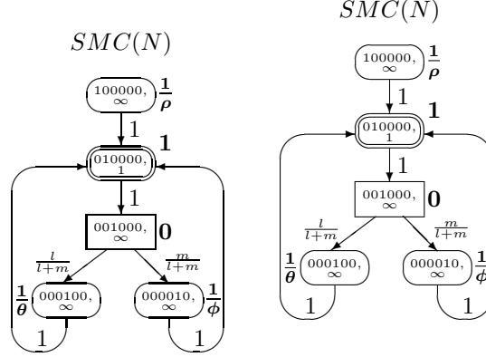
FIG. 2. The underlying SMC of N = \text{Box}_{\text{dtsd}}(\overline{E}) for E = [(\{a\}, \rho) * ((\{b\}, \natural_k^1); (((\{c\}, \natural_l^0); (\{d\}, \theta)) \square (((\{e\}, \natural_m^0); (\{f\}, \phi)))) * \text{Stop}]
