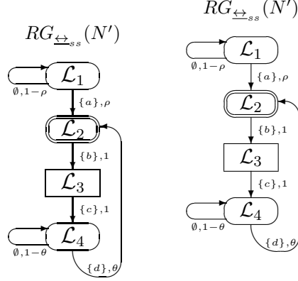
FIG. 5. The quotient reachability graph of N' = \text{Box}_{dtsd}(\bar{F}) for F = [(\{a\}, \rho) * ((\{b\}, \mathfrak{h}_k^1); (((\{c\}, \mathfrak{h}_l^0); (\{d\}, \theta)_1) \square ((\{c\}, \mathfrak{h}_m^0); (\{d\}, \theta)_2))) * \text{Stop}]
