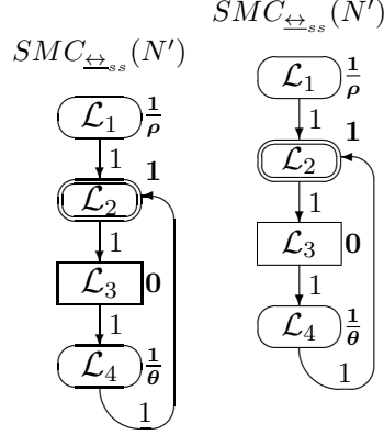
FIG. 7. The quotient underlying SMC of N' = \text{Box}_{\text{dtsd}}(\overline{F}) for F = [(\{a\}, \rho) * ((\{b\}, \mathfrak{h}_k^1); (((\{c\}, \mathfrak{h}_l^0); (\{d\}, \theta)_1) \parallel ((\{c\}, \mathfrak{h}_m^0); (\{d\}, \theta)_2))) * \text{Stop}]
