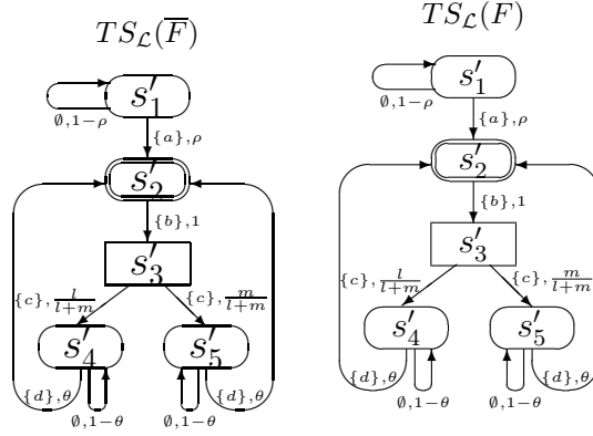
FIG. 3. The multi-action transition system of \bar{F} for F = [(\{a\}, \rho) * ((\{b\}, \mathfrak{b}_k^1); (((\{c\}, \mathfrak{b}_l^0); (\{d\}, \theta)_1) \sqcup ((\{c\}, \mathfrak{b}_m^0); (\{d\}, \theta)_2))) * \text{Stop}]
