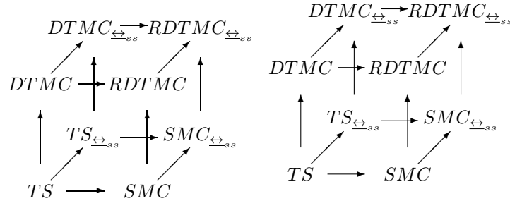
FIG. 11. The cube of interrelations for the standard and quotient transition systems and Markov chains of the process expressions
