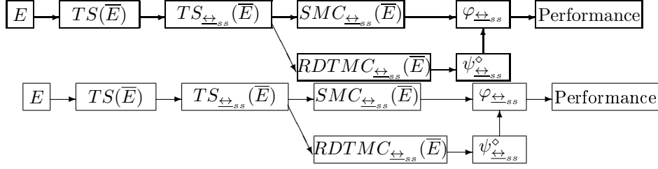
FIG. 12. Equivalence-based simplification of performance evaluation
