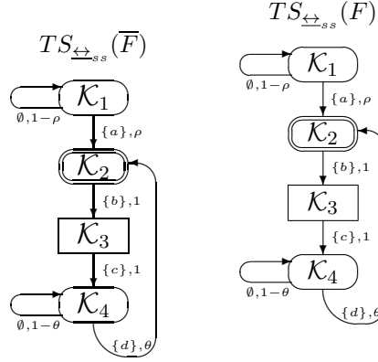
FIG. 4. The quotient transition system of \bar{F} for F = [(\{a\}, \rho) * ((\{b\}, \mathfrak{z}_k^1); (((\{c\}, \mathfrak{z}_l^0); (\{d\}, \theta)_1) \square ((\{c\}, \mathfrak{z}_m^0); (\{d\}, \theta)_2))) * \text{Stop}]
