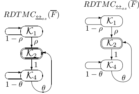
FIG. 9. The reduced quotient DTMC of \bar{F} for F = [(\{a\}, \rho) * ((\{b\}, \mathfrak{h}_k^1); (((\{c\}, \mathfrak{h}_l^0); (\{d\}, \theta)_1) \square ((\{c\}, \mathfrak{h}_m^0); (\{d\}, \theta)_2))) * \text{Stop}]
