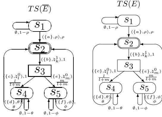
FIG. 1. The transition system of \bar{E} for E = [(\{a\}, \rho) * ((\{b\}, h_k^1); (((\{c\}, h_l^0); (\{d\}, \theta)) [((\{e\}, h_m^0); (\{f\}, \phi)))) * \text{Stop}]
