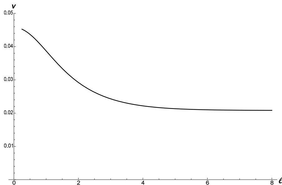
FIG. 6. Graph of the normalized volume of a tetrahedron T
