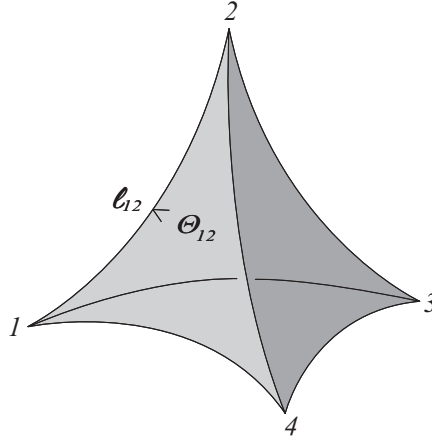
FIG. 1. A hyperbolic tetrahedron
