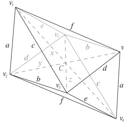
FIG. 2. An antipodal octahedron \mathcal{O}(a, b, c, d, e, f)
