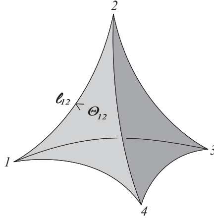
FIG. 1. A hyperbolic tetrahedron
