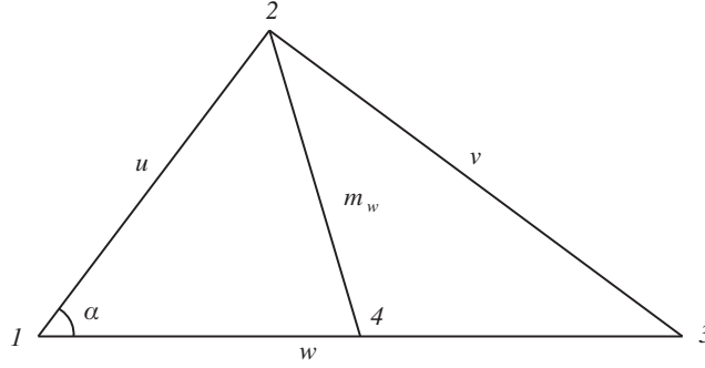
FIG. 3. Compact hyperbolic triangle \Delta(u, v, w) .
