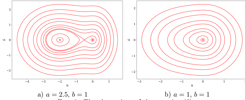
FIG. 1. The phase plane of the equation (6)
