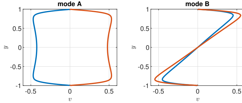
FIG. 4. Unstable modes v(y) . Blue – real part, orange – imaginary part. Re = 5000 , \beta = 0.77 , W = 3 , \omega = 1 , \zeta = 0 .
