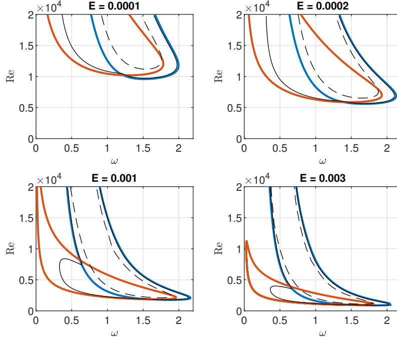
FIG. 8. Neutral stability curves. Blue line for a mode A , orange line for a mode B , \zeta = 0 . Solid black line is \zeta = 0.1 , dashed black line is \zeta = 0.3 . \beta = 0.77 .
