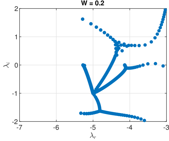
FIG. 9. Fragment of the spectrum at \text{Re} = 5000 , W = 0.2 , \beta = 0.77 , \omega = 1 , \zeta = 0 .
