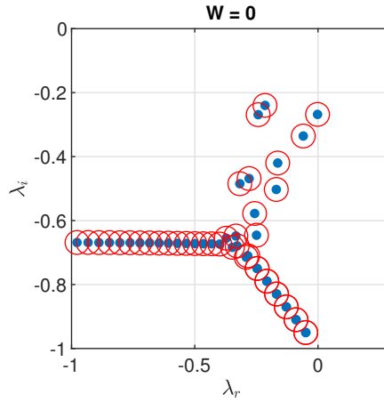
FIG. 2. Spectra of Orr-Sommerfeld equation (red circles) and mVP model at W = 0 (blue dots). Re = 5000 , \beta = 0.77 , \omega = 1 , \zeta = 0 .
