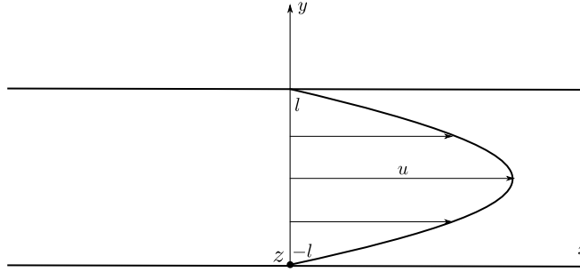
FIG. 1. Flow in the plane channel.
