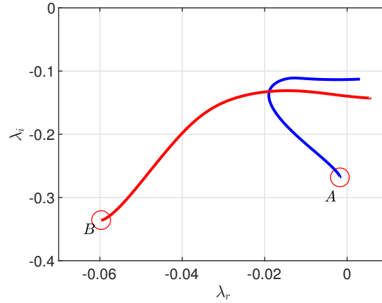
FIG. 5. Trajectories of eigenvalues A and B from W = 0 to W = 3 . Re = 5000 , \beta = 0.77 , \omega = 1 , \zeta = 0 .
