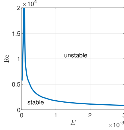
FIG. 6. Zones of stability and instability, \text{Re} - E plane, \beta = 0.77 .
