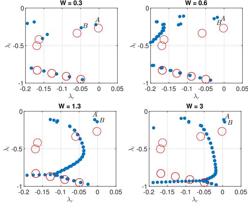
FIG. 3. Spectra of mVP with various W . Red circles are the positions of eigenvalues at W = 0 . Re = 5000 , \beta = 0.77 , \omega = 1 , \zeta = 0 .
