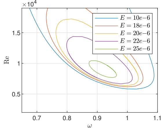
FIG. 7. Neutral stability curves of mode A , \beta = 0.77 , \zeta = 0 .
