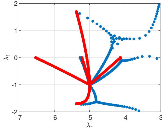
FIG. 10. Numerical spectrum (blue) and solution of (23) (red). Re = 5000 , W = 0.2 , \beta = 0.77 , \omega = 1 , \zeta = 0 .
