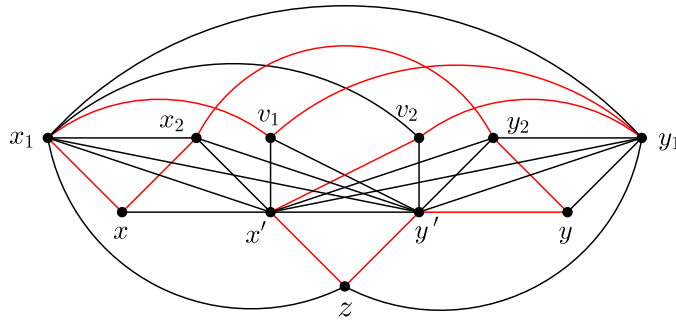
FIG. 3. Hamiltonian cycle of graph F_{11}^2 \in \mathcal{F}_{11,3,\Delta}
