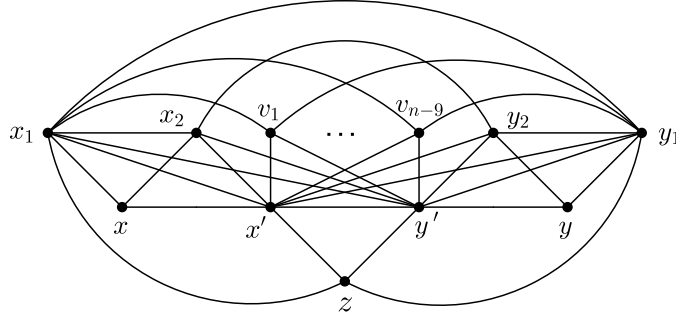
FIG. 2. Graph F_n^2
