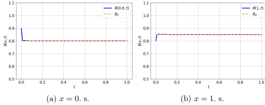
FIG. 3. Temperature profile at observed points on the boundaries.
