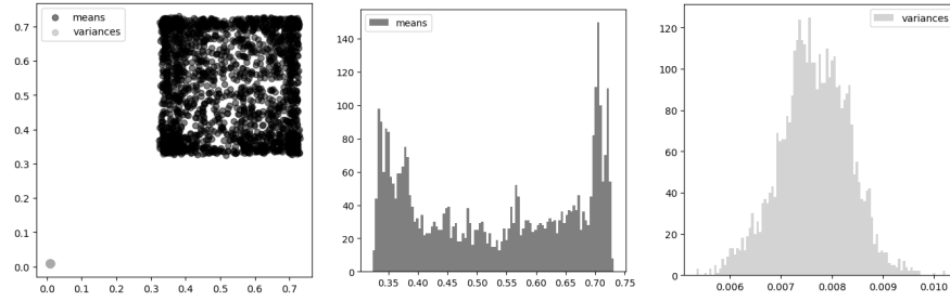
FIG. 8. The result of procedure application on white noise and seasonality data presented by (17). On the left – scatter plot of Y_{mns} and Y_{vrs} ; in the middle – histogram for Y_{mns} ; on the right – histogram for Y_{vrs}
