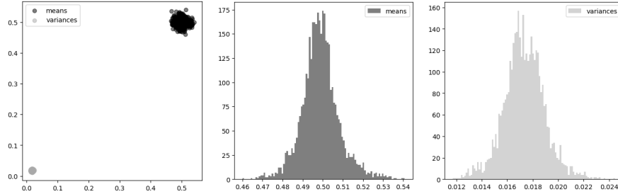
FIG. 6. The result of procedure application on white noise data represented by (13). On the left – scatter plot of Y_{mns} and Y_{vrs} ; in the middle – histogram for Y_{mns} ; on the right – histogram for Y_{vrs}
