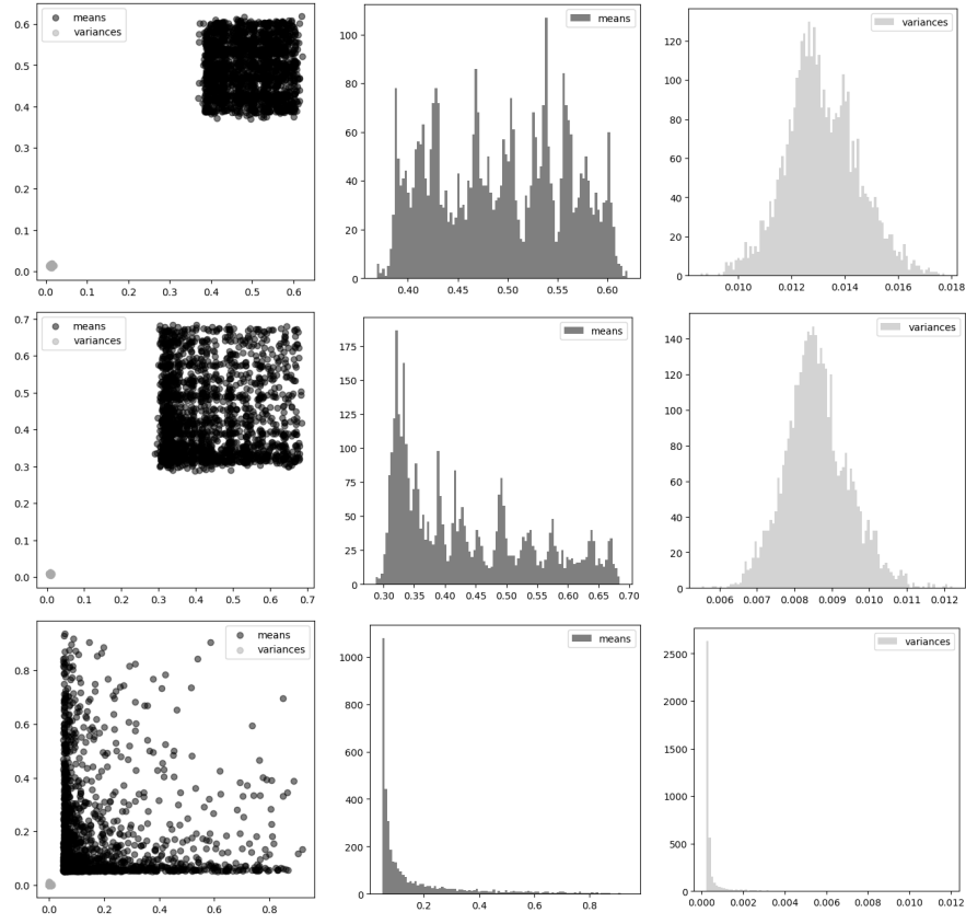
FIG. 7. The result of procedure application on white noise with trend data presented by equations (14) (first line), (15) (second line), (16) (third line). On the left – scatter plot of Y_{mns} and Y_{vrs} ; in the middle – histogram for Y_{mns} ; on the right – histogram for Y_{vrs}
