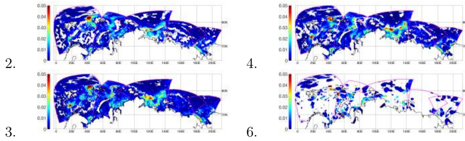
FIG. 11. 9 clusters partition. Eddy kinetic energy (27) of clusters 2-4 and 6: the geographic distribution of the vertically averaged eddy kinetic energy for clustering with six clusters.
