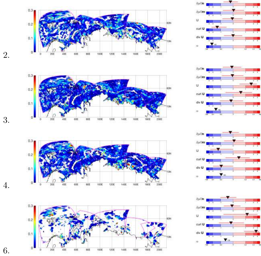
FIG. 9. Weighted average clustering with 9 clusters. Clusters 2-4 and 6: the geographic distribution of the vertically averaged coefficient of determination value (left column) and the average deviation of large-scale characteristics for each cluster relative to its overall mean in terms of the standard deviation of that characteristic (right column). The horizontal red lines at the top of each panel in the right column indicate the standard deviation range of the characteristics for each cluster. The last panel shows only the mean value of the angle \alpha without reference to its overall mean and without the standard deviation.
