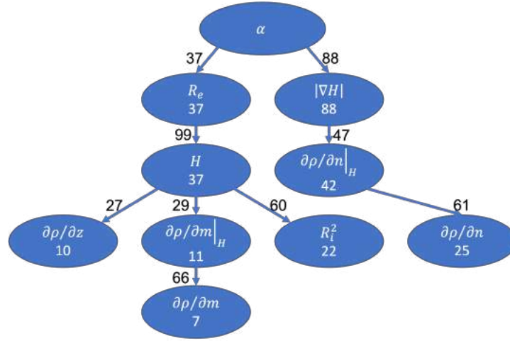
FIG. 1. A system of interdependent characteristics with a correlation ratio of at least 25% based on the results of calculations for the Barents Sea. The numbers express the percentage of the correlation level: in the case of arrows – between the connected characteristics, in the case of the characteristics themselves – between the characteristic and \alpha .
