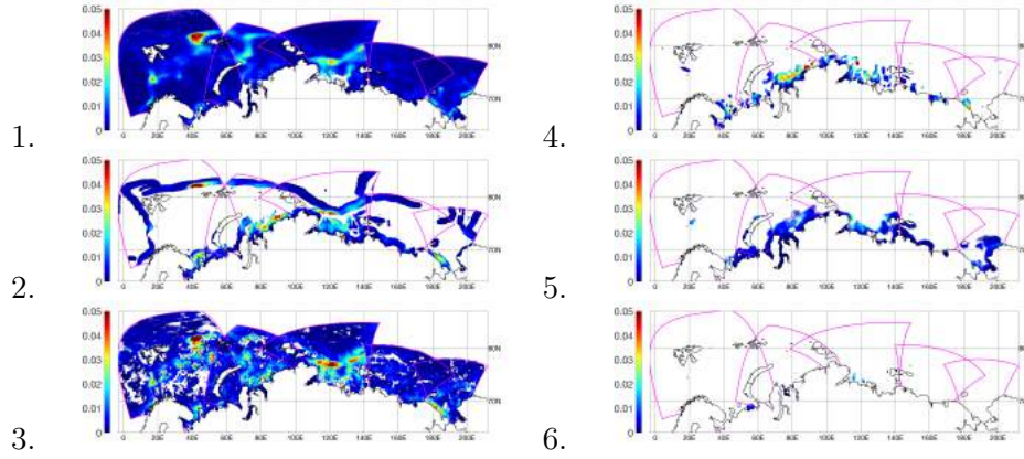
FIG. 6. Eddy kinetic energy (27): the geographic distribution of the vertically averaged eddy kinetic energy for clustering with six clusters.
