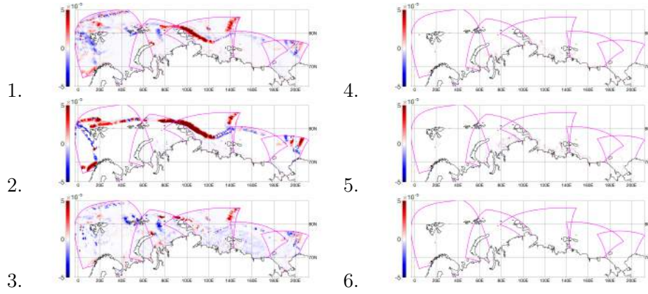
FIG. 7. Baroclinic generation rate of EKE (28): the geographic distribution of the vertically averaged baroclinic generation rate of EKE for clustering with six clusters.
