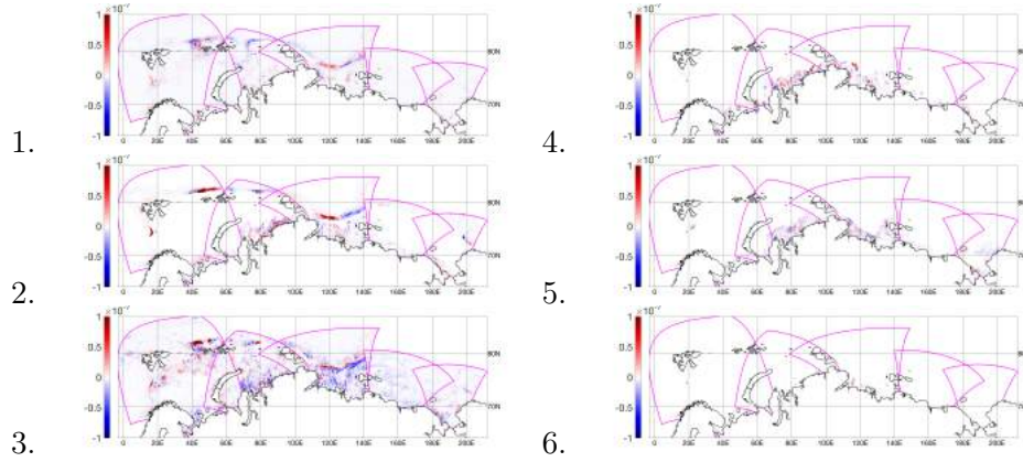
FIG. 8. Barotropic generation rate of EKE (29): the geographic distribution of the vertically averaged barotropic generation rate of EKE for clustering with six clusters.
