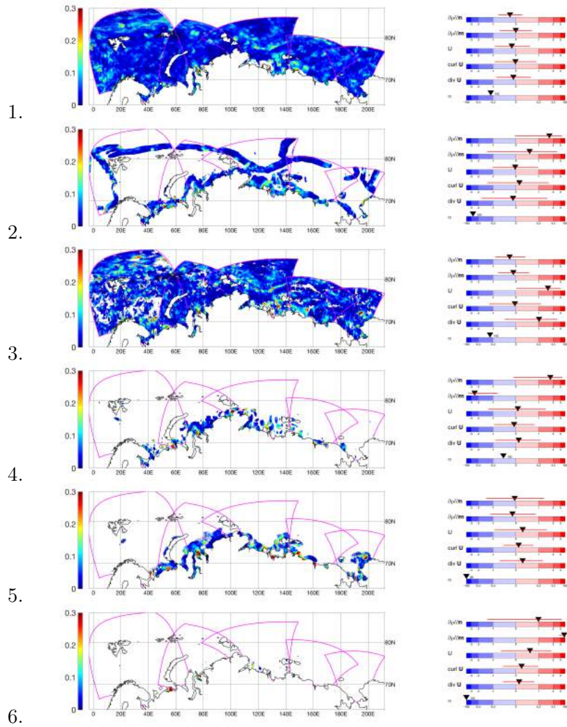
FIG. 4. Weighted average clustering with 6 clusters: the geographic distribution of the vertically averaged coefficient of determination value (left column) and the average deviation of large-scale characteristics for each cluster relative to its overall mean in terms of the standard deviation of that characteristic (right column). The horizontal red lines at the top of each panel in the right column indicate the standard deviation range of the characteristics for each cluster. The last panel shows only the mean value of the angle \alpha without reference to its overall mean and without the standard deviation.
