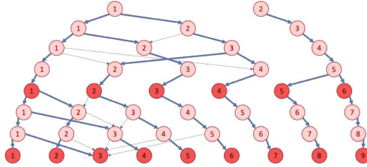
FIG. 3. Geneological tree of inheritance of cluster properties when their number increases from 2 to 9. Bold arrows indicate which cluster from the previous partition the center of the subsequent partition cluster would belong to. Thin arrows indicate connections with other closest clusters, that is, with those whose distance to the center is no more than 2 times greater than the distance to the parent cluster. Clusters of 6 and 9-cluster partitions are highlighted in dark red.
