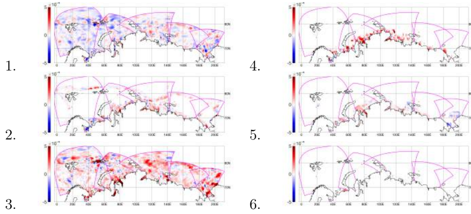
FIG. 5. Eddy mass flux (4): the geographic distribution of the vertically averaged eddy mass flux for clustering with six clusters.
