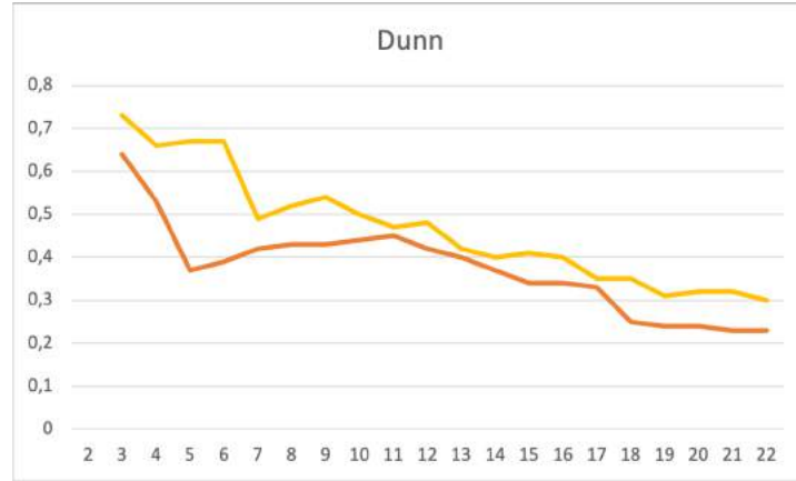
FIG. 2. Optimal Dunn index [12] for clusterization with different numbers of clusters: with account of determination coefficient (yellow line), and without it (red line).
