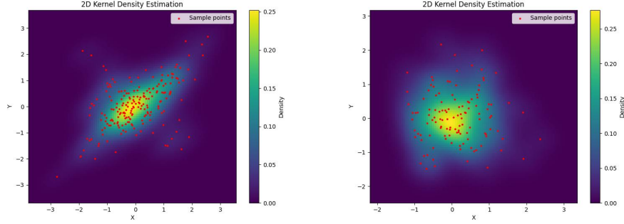
FIG. 10. 2D projected density estimation for \tilde{t}(1) (left) and ci \tilde{t}(1) (right) for base dimension 40
