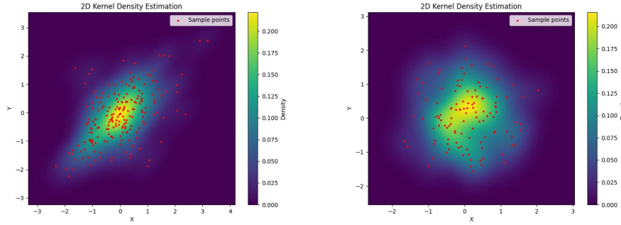
FIG. 9. 2D projected density estimation for \tilde{t}(2) (left) and ci \tilde{t}(2) (right) for base dimension 40
