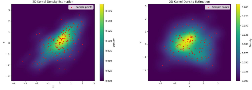
FIG. 2. 2D projected density estimation for \tilde{t}(4) (left) and ci \tilde{t}(4) (right) for base dimension 20
