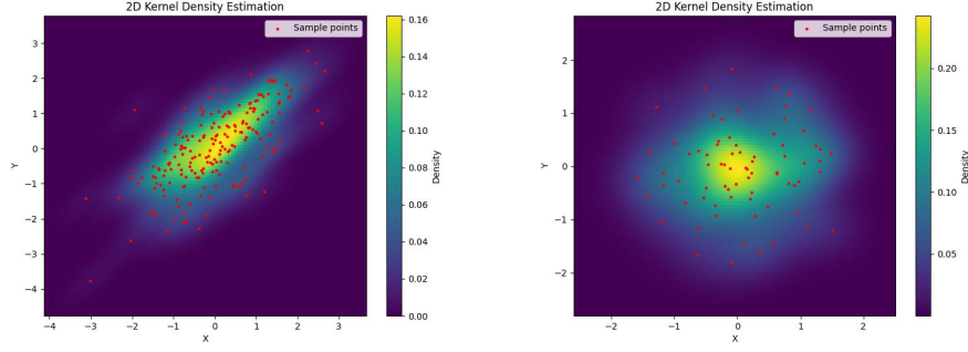
FIG. 7. 2D projected density estimation for \tilde{t}(8) (left) and ci \tilde{t}(8) (right) for base dimension 40
