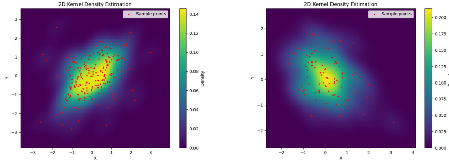
FIG. 8. 2D projected density estimation for \tilde{t}(4) (left) and ci \tilde{t}(4) (right) for base dimension 40
