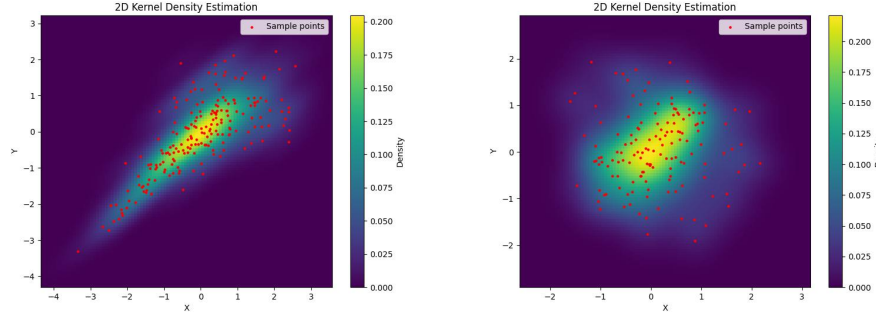
FIG. 6. 2D projected density estimation for vine (left) and ci \ vine (right) for base dimension 20
