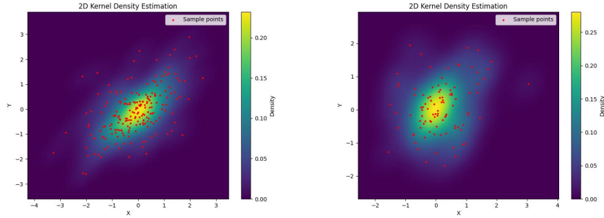
FIG. 11. \widetilde{Laplace} projected density estimation for \widetilde{Laplace} (left) and ci \widetilde{Laplace} (right) for base dimension 40
