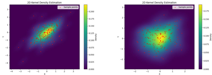
FIG. 1. 2D projected density estimation for \tilde{t}(8) (left) and ci \tilde{t}(8) (right) for base dimension 20
