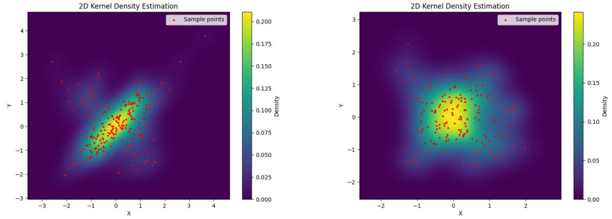
FIG. 4. 2D projected density estimation for \tilde{t}(1) (left) and ci \tilde{t}(1) (right) for base dimension 20
