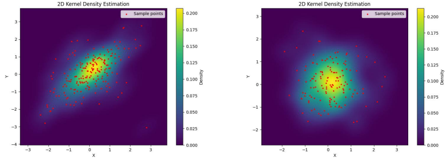
FIG. 3. 2D projected density estimation for \tilde{t}(2) (left) and ci \tilde{t}(2) (right) for base dimension 20
