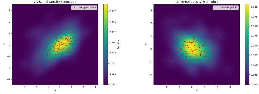
FIG. 5. 2D projected density estimation for \widetilde{Laplace} (left) and ci \widetilde{Laplace} (right) for base dimension 20
